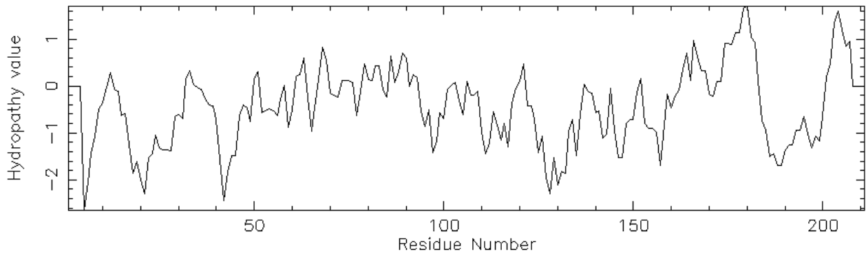
Hydropathy plot of residues 1 to 211 of sequence dbAMP-09977 using OHM Hydropathy parameters (Sweet & Eisenberg)
