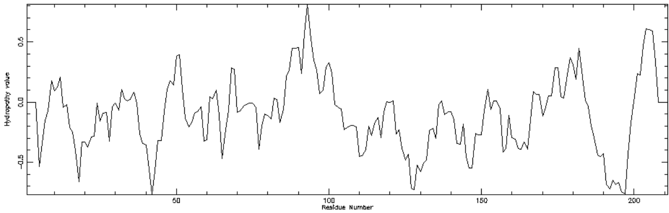
Hydropathy plot of residues 1 to 211 of sequence dbAMP-09977 using Consensus parameters (Eisenberg et al)
